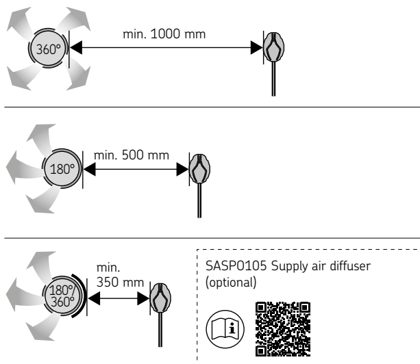
Figure 13. Minimum distance from the supply air vent to the temperature sensor
