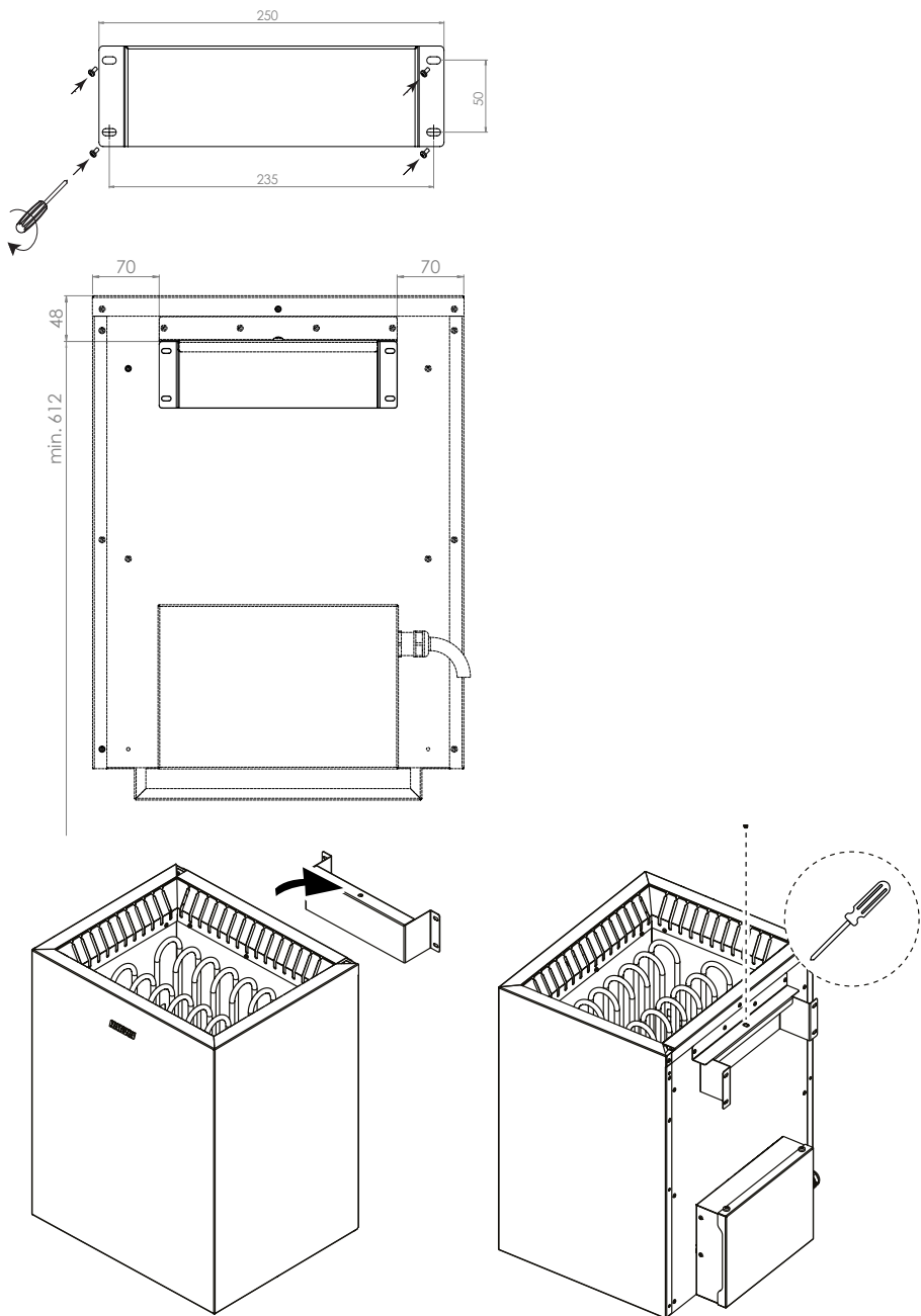
Figure 2. Sauna heater installation
