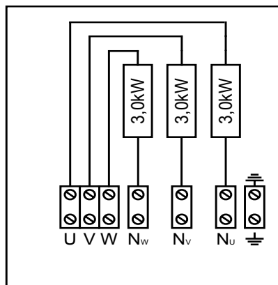
Figure 8. Wiring diagram HLW90E
