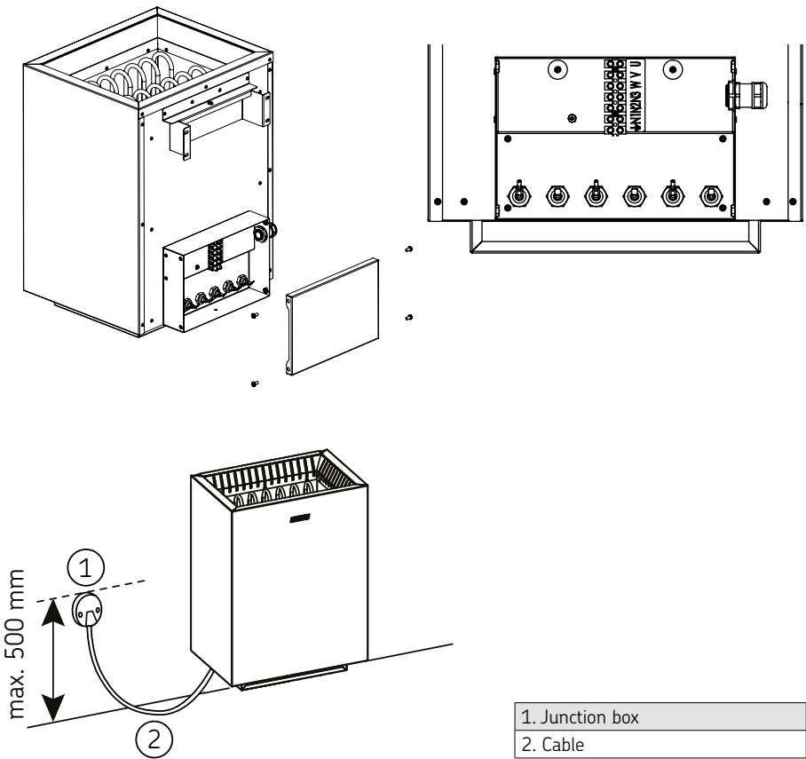
Figure 4. Electrical connections
