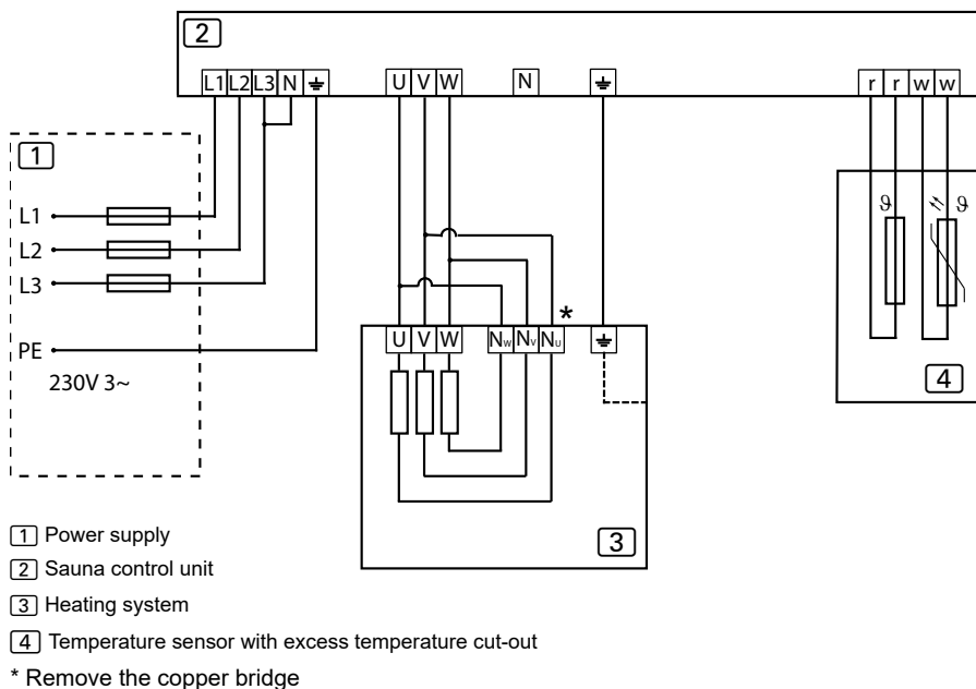
Figure 11. Connection diagram 230V 3~
