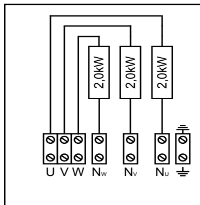
Figure 6. Wiring diagram HLW60E
