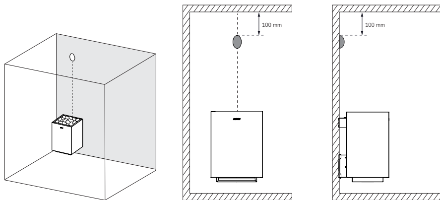
Figure 3. Installing the heat sensor on the wall
