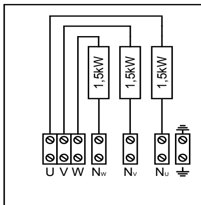
Figure 5. Wiring diagram HLW45E
