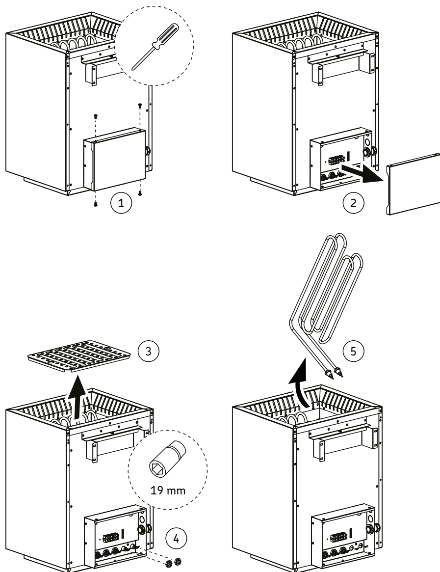
Figure 14. Changing of heating elements
