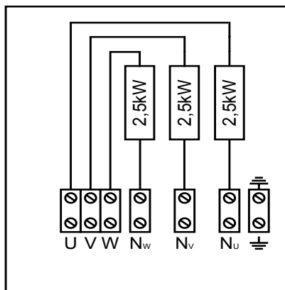
Figure 7. Wiring diagram HLW75E
