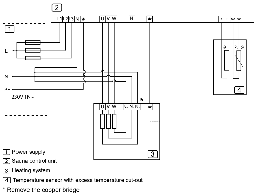
Figure 10. Connection diagram 230V 1N~
